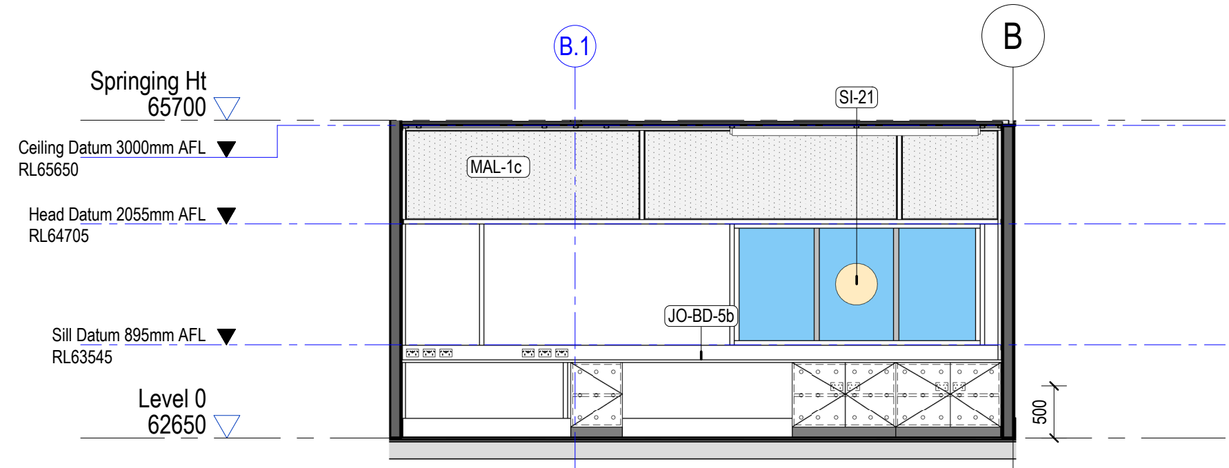
4 0.11 - Training 02 - South Elevation 1 : 50
