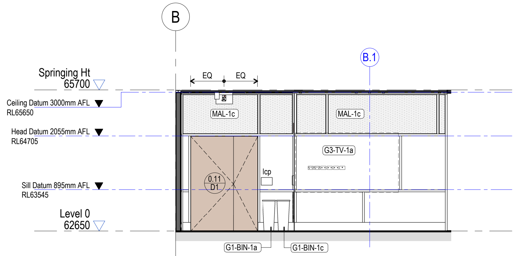
2 0.11 - Training 02 - North Elevation 1 : 50
