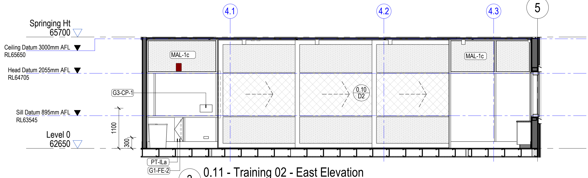
3 0.11 - Training 02 - East Elevation 1 : 50
