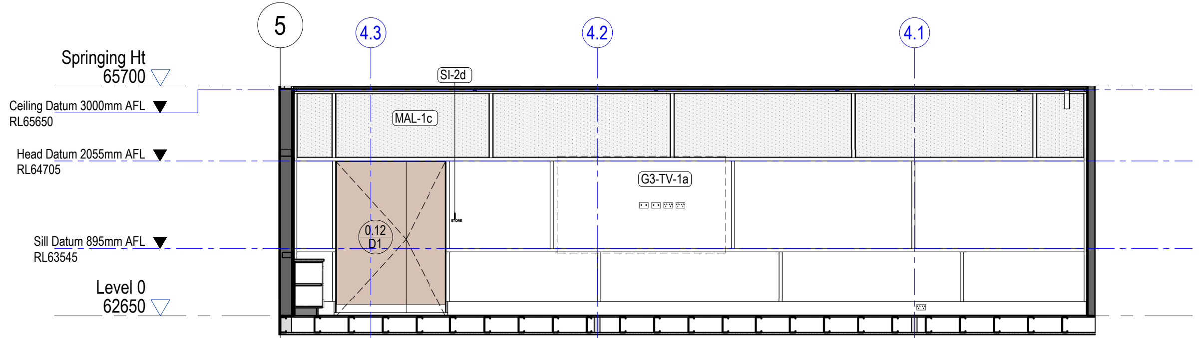
5 0.11 - Training 02 - West Elevation 1 : 50
